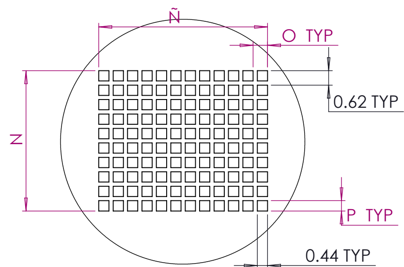
TYPICAL VENT PATTERN 0.44 SQ. HOLES (10) VERT. X (12) HORZ.
